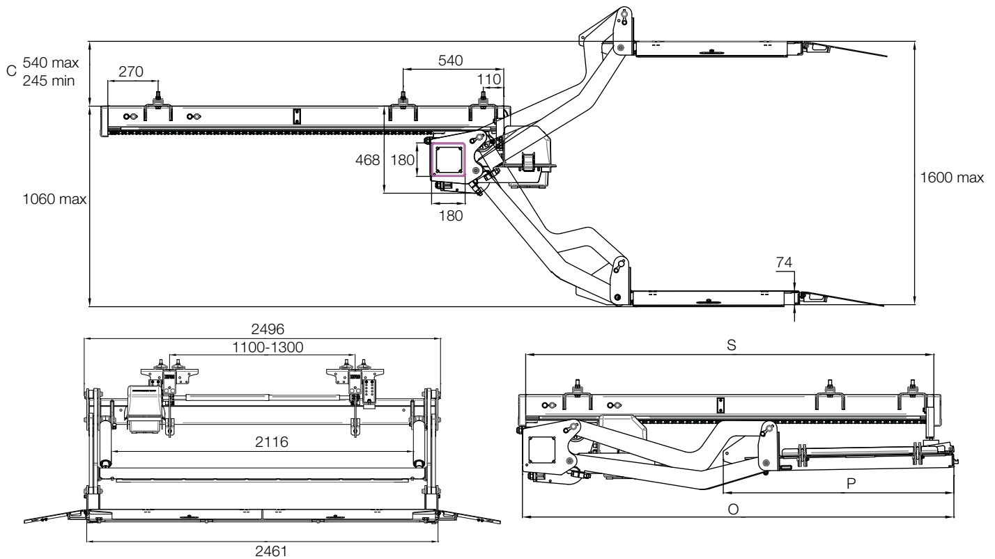
Installation dimensions (mm)
