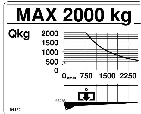
Loading diagram
