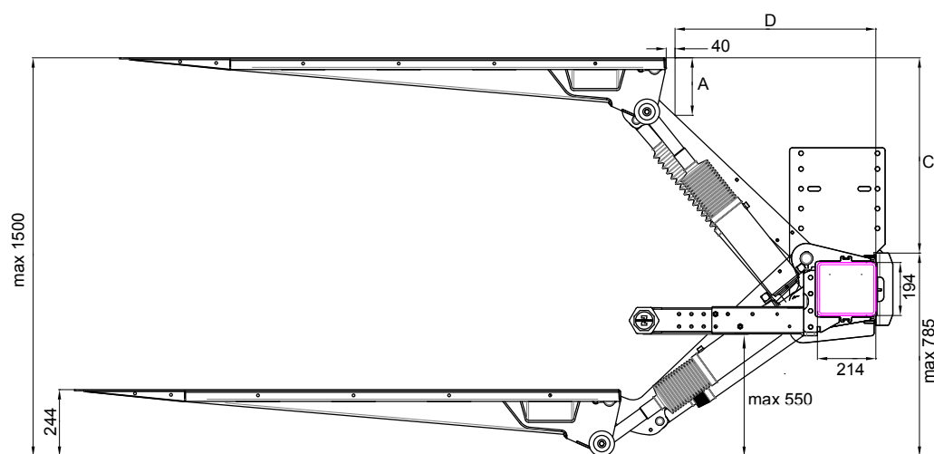
Installation dimensions (mm)
