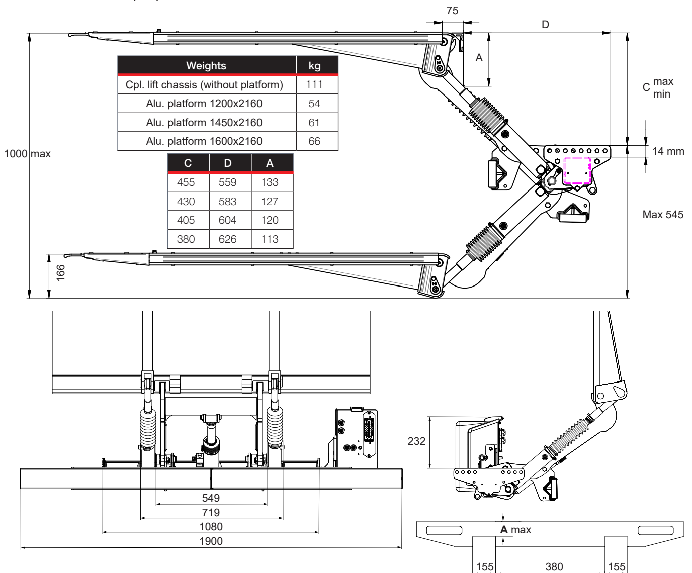
Installation dimensions (mm)
