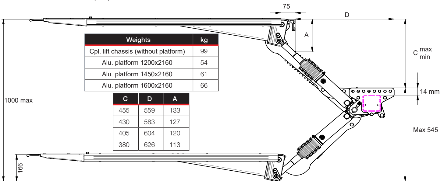
Installation dimensions (mm)
