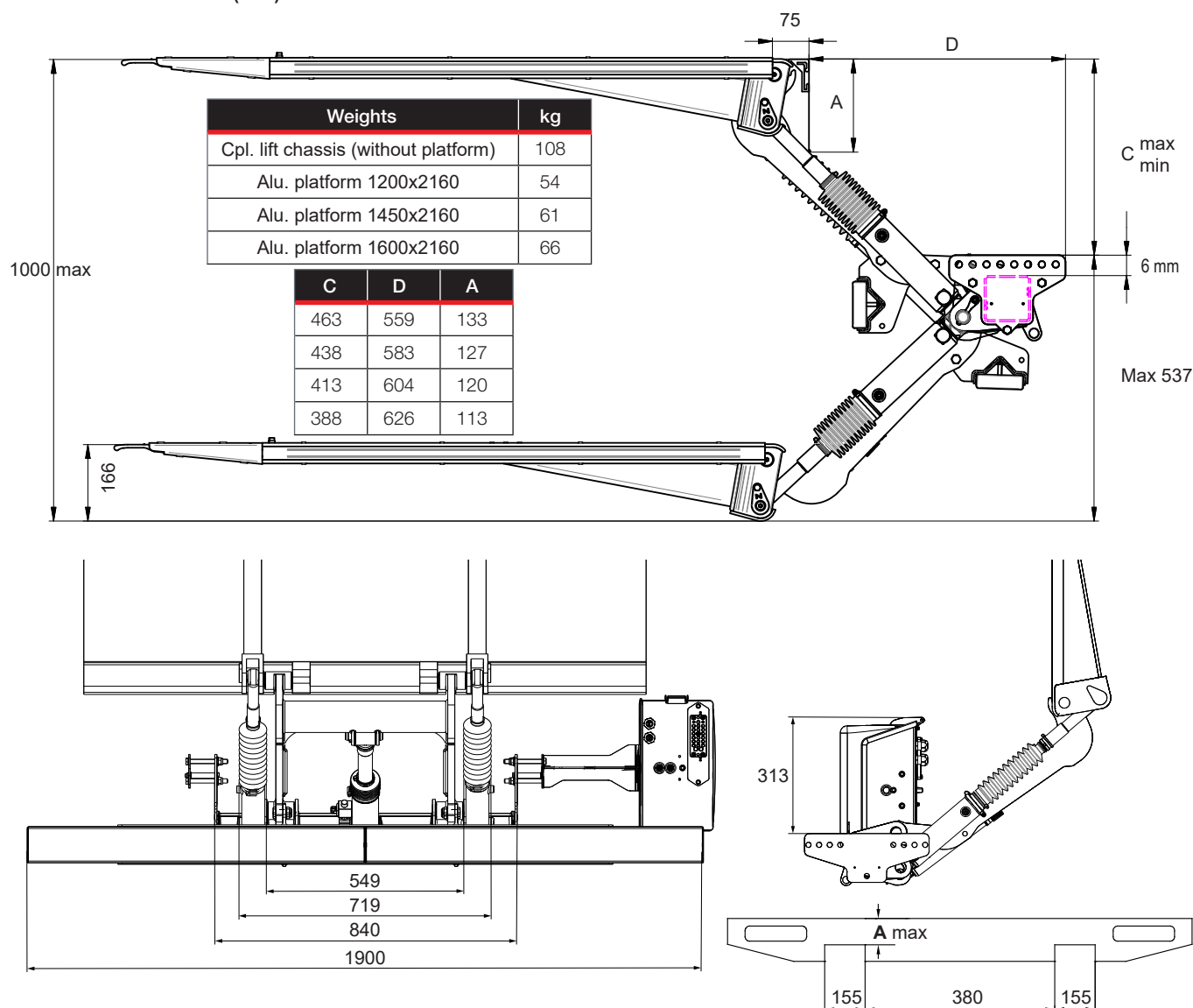
Installation dimensions (mm)
